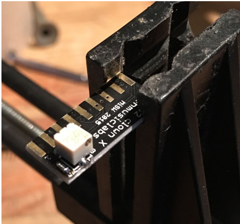
Now fit the 50K trimmer (mouser 3223J-1-503ECT-ND)
