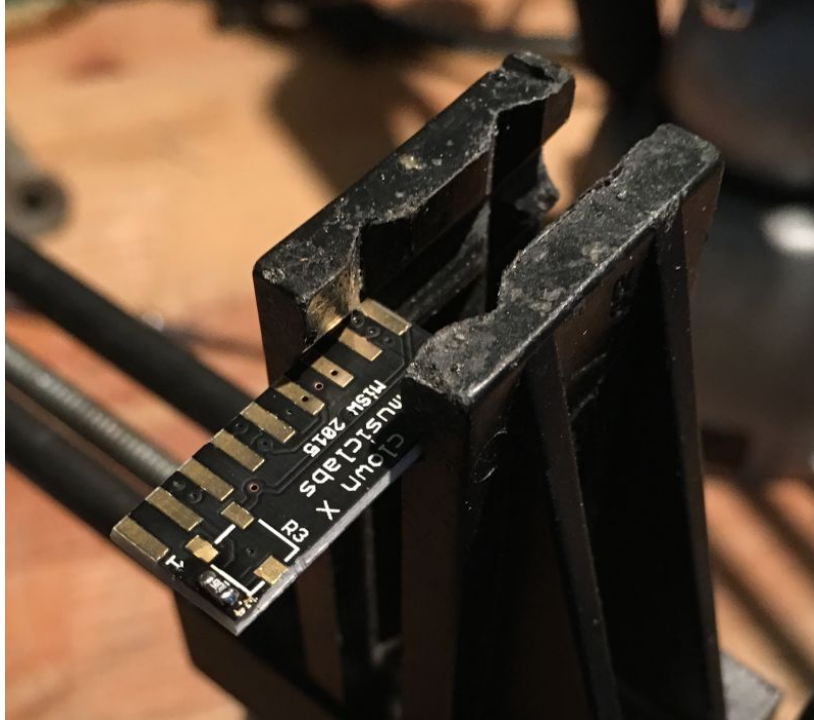
First fit the 10M chip resistor (mouser 311-10MGRCT-ND)
