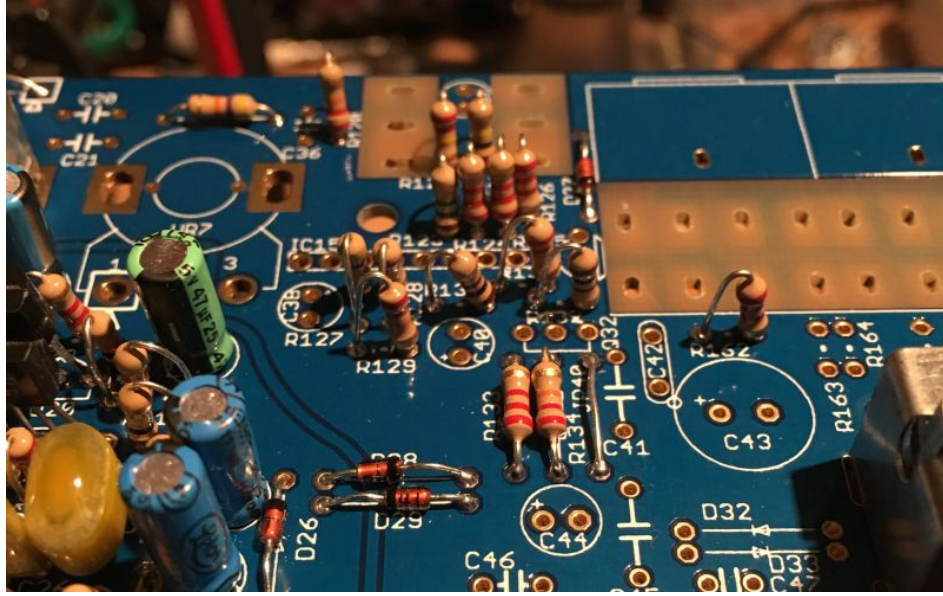
Fit the diodes and resistors.
