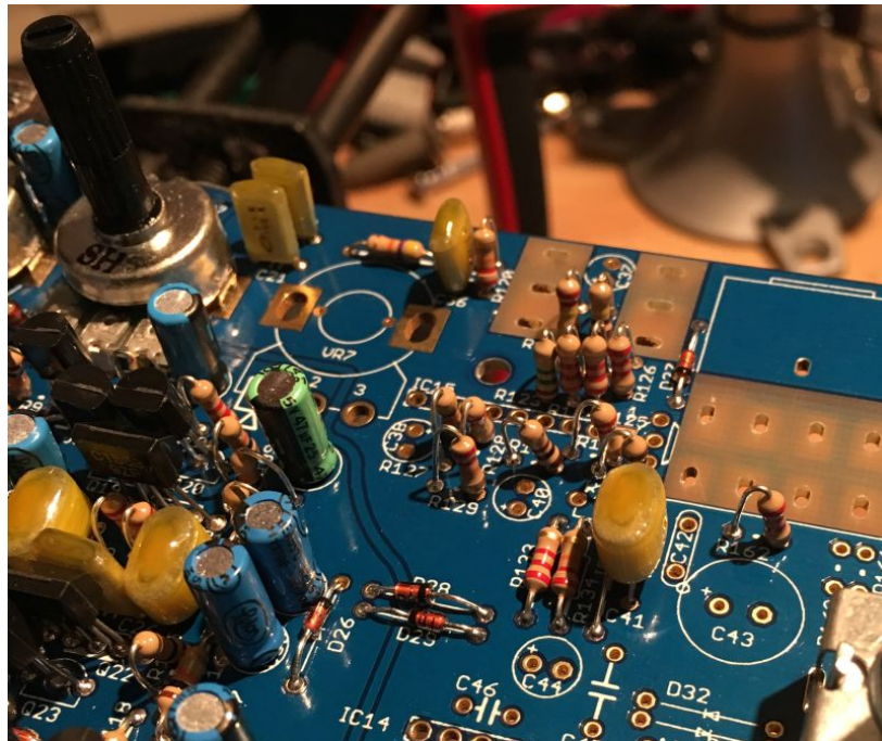
Fit the metal film capacitors.
