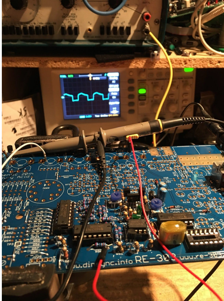
The picture shows me reading the square waveform from Q8 pin 2
