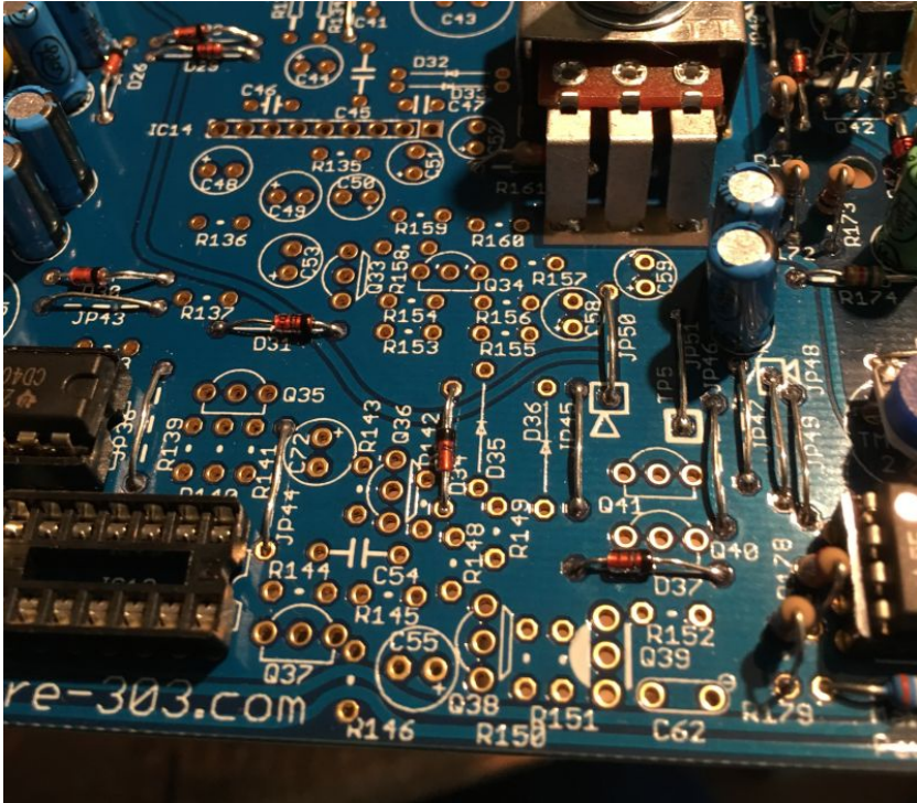
Fit the diodes.
