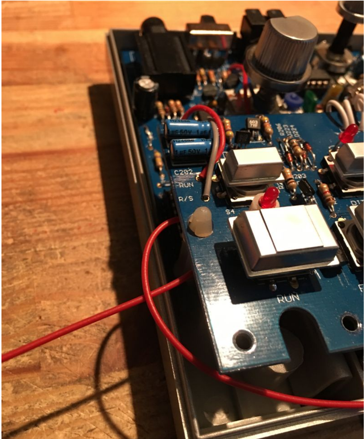
And around the other standoff
