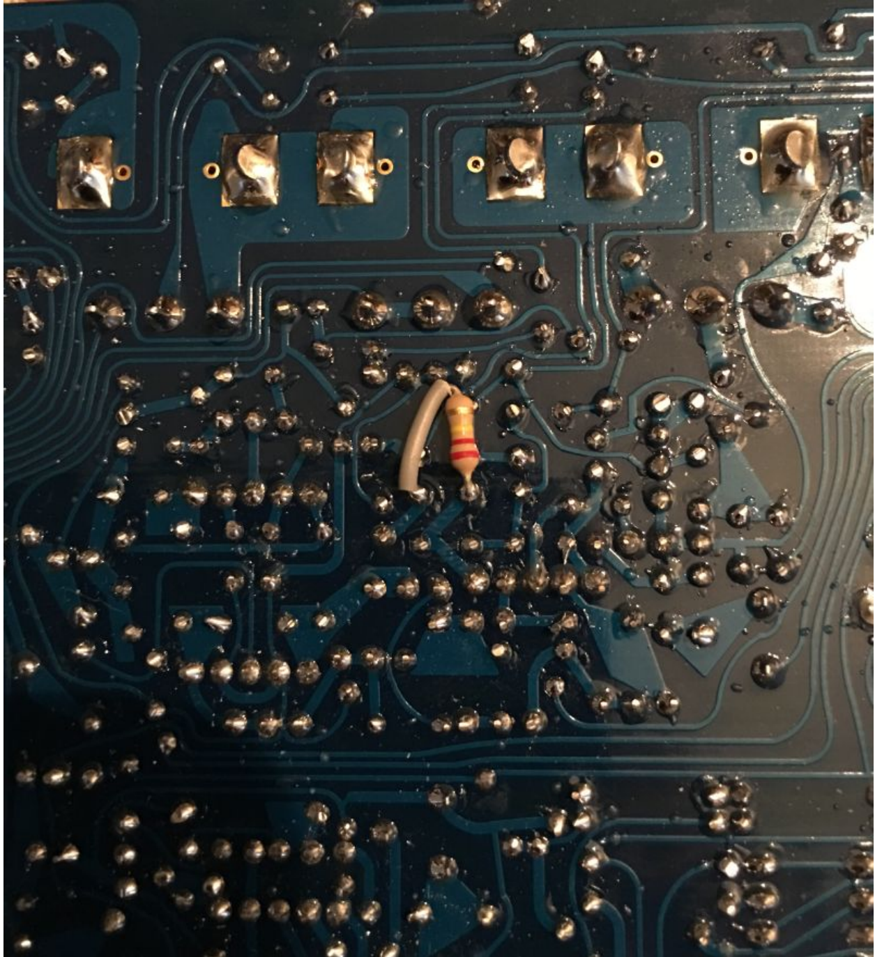
220K resistor in parallel with R97
